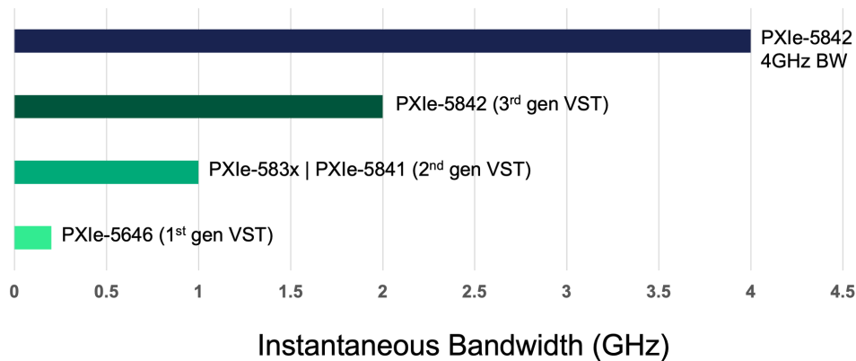
FIGURE 2 Instantaneous RF Bandwidth in GHz of NI VST Models
