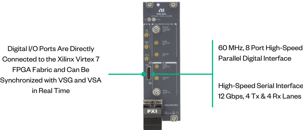
FIGURE 7 Digital Interfacing Ports on the PXle-5841 Front Panel
