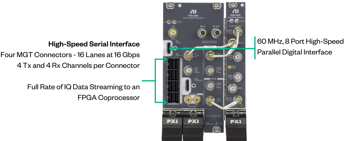
FIGURE 8 Digital Interfacing Ports on the PXle-5842 Front Panel
